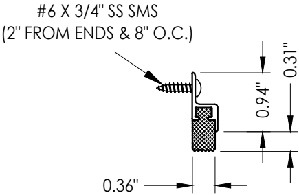
6 PERIMETER SEAL NGP 165 N-S
