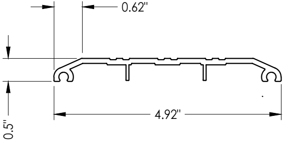
39 ADA THRESHOLD NGP 425E
