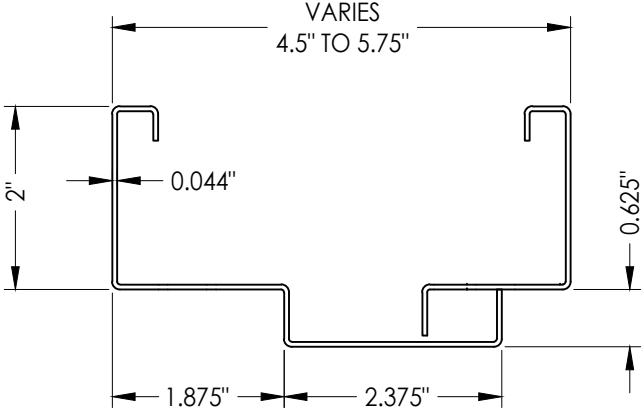
2 ADJUSTABLE METAL FRAME 18 GA.
