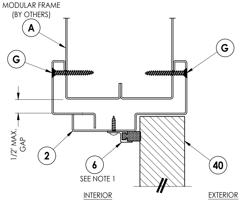
1 4 VERTICAL CROSS SECTION Modular Frame Installation
